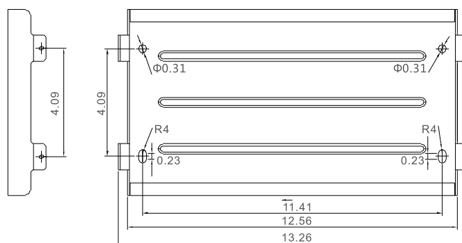
Figure 5.Mounting bracket dimensions
