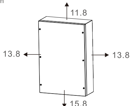
Figure 3.Installation Space Requirement
