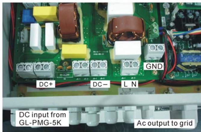
GCI-5K grid tie inverter pin outs
